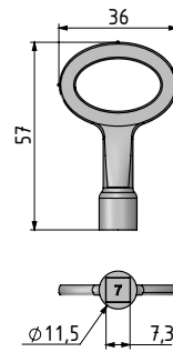
26727 7mm Kare
